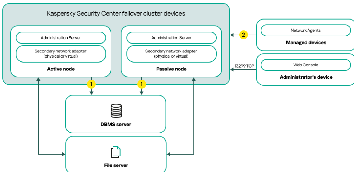
A scheme that uses a secondary network adapter
